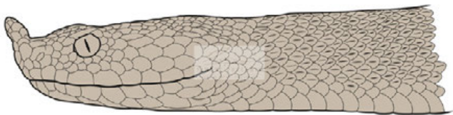
Vipera ammodytes
